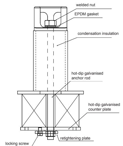
Fastening to wooden roof
