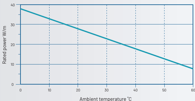
Rated power W/m at different temperatures
